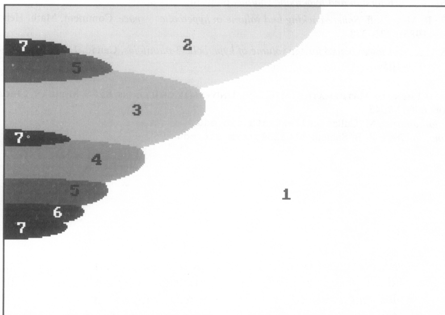
FIGURE 2. Power m \leq 7 yielding the largest volume tube.
