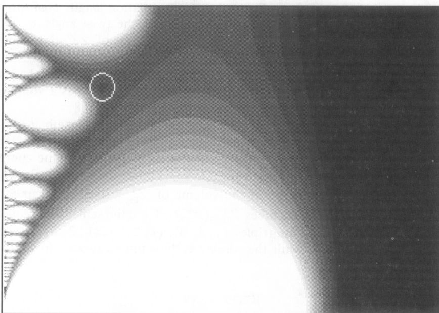
FIGURE 1. The volume of Z_{\log 3}(x)/\langle x \rangle as a function of complex length.
